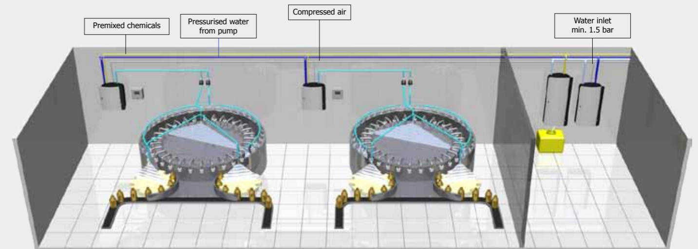
Centralised solution: A chemical pump station supplies each work station with premixed chemicals. Ensures uniform concentration.
