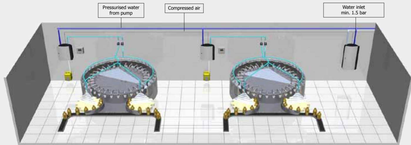
Decentralised solution: Chemicals are located at each work station. Individual dosing possible.
